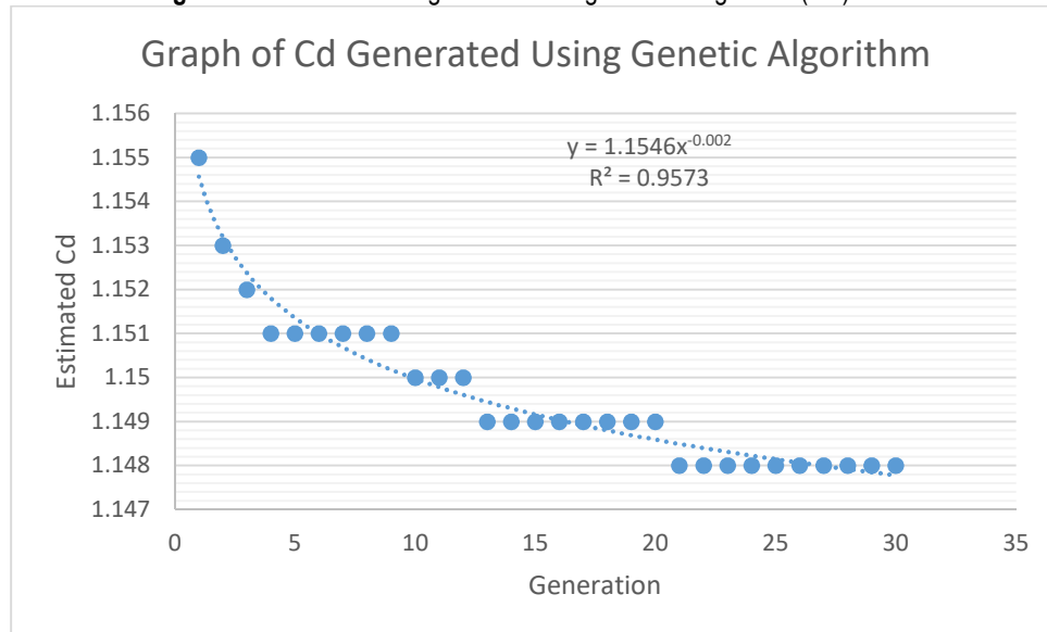
Figure 12: Relation of Cd Generated using Genetic Algorithm(GA) model
