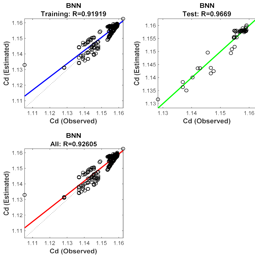
Figure 14: Distribution diagram of the observational-computational values in training and testing stages of Bayesian Neural Network (BNN) Model varification of Cd.
