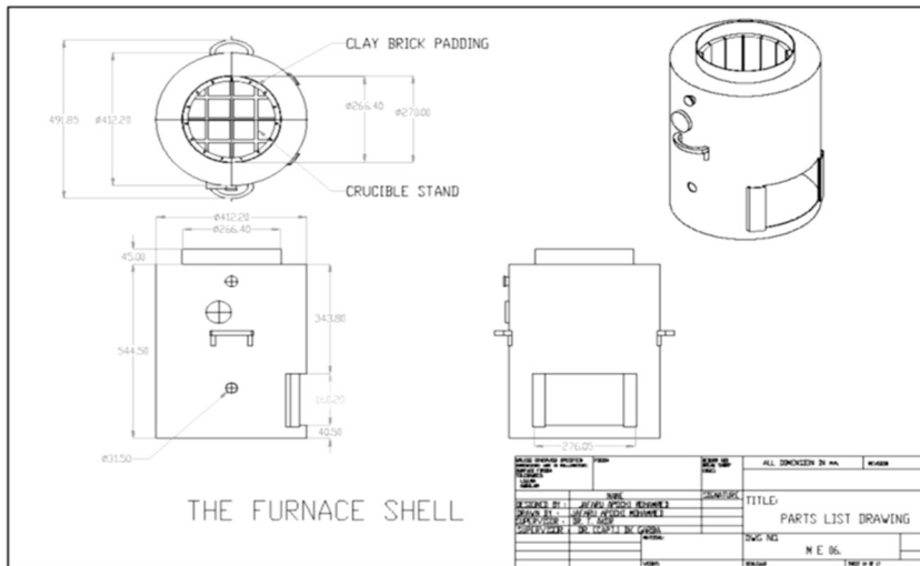
Plate 2: Specification for the furnace's shell and door.
