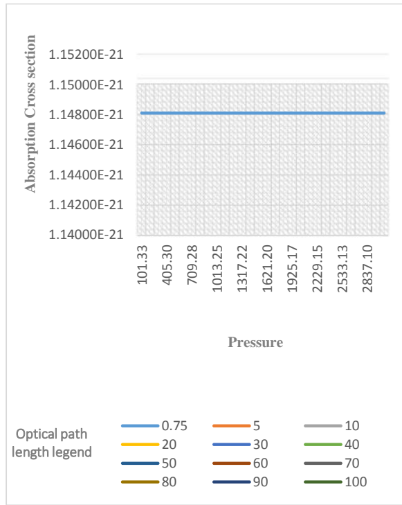
Figure 0.2 effects of pressure and optical path length on the OACS at 255.442 nm. Based on the values of the transmittances obtained, the OACS was determined and graphically presented as shown in Figure 4.2 clearly. The OACS was found to maintain a constant value of 1.148E - 21 \text{ cm}^2/\text{molecule} as the pressure and OPL increased from 101.33 – 3039.75 mbar and 0.75 – 130 cm respectively. This report shows that pressure and OPL variation have zero effects on the OACS which is consistent with the work of [16] who reported the independence of pressure (0.1 to 3.0 atm) on OACS at 255.442 nm and an OPL of 20 cm.
