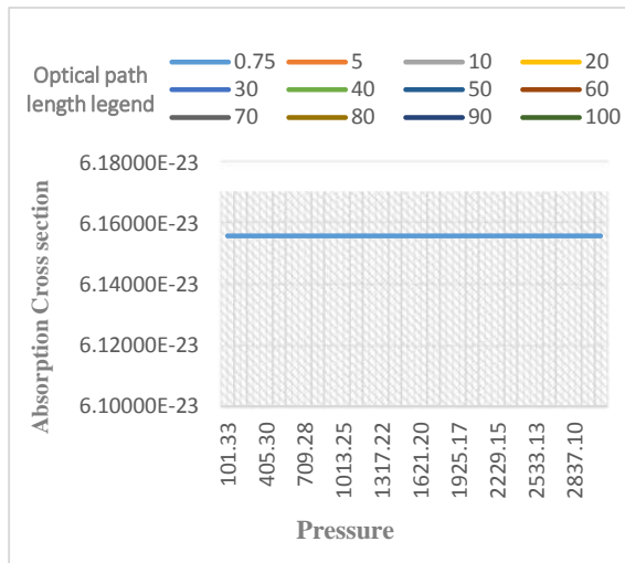
Figure 0.4 effects of pressure and optical path length on the OACS at 296.73 nm
