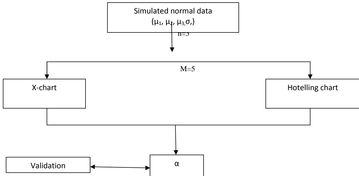
Fig.1 Simulated procedure (Type 1 Error probability)
