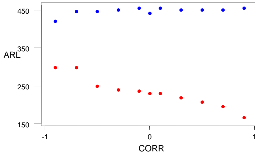
Fig .5 : ARL of Type I Error for Average of Univariates and Multivariate
