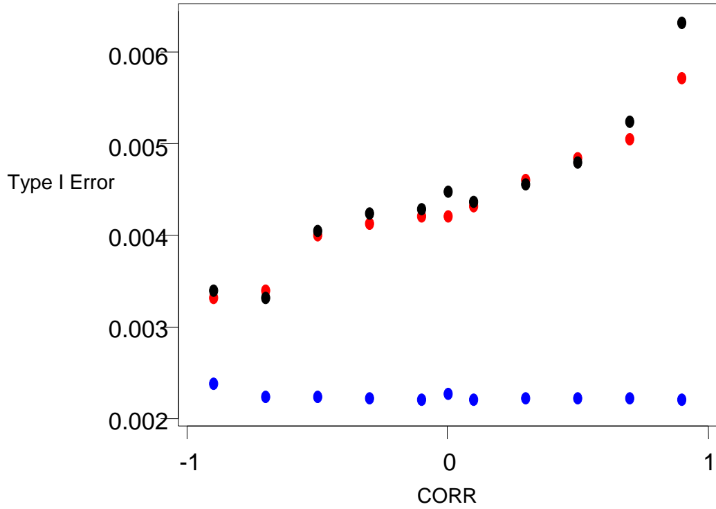
Fig 2 :Type I Error Probability of univariates and Multivariate
