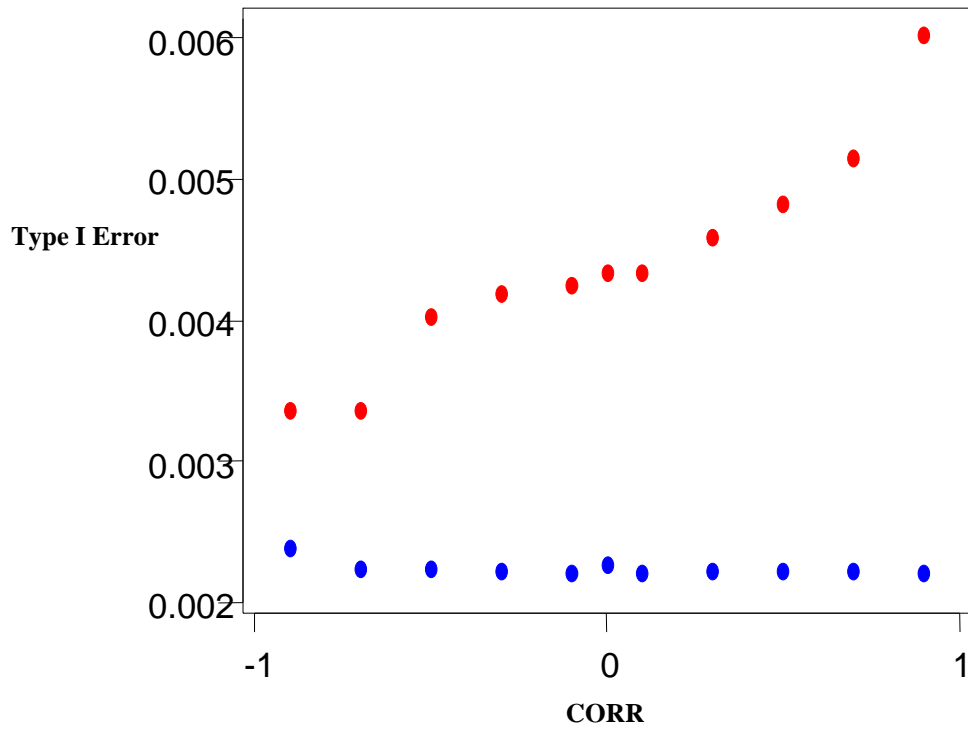
Fig 3: Type I Error Probability for average of Univariates and Multivariate
